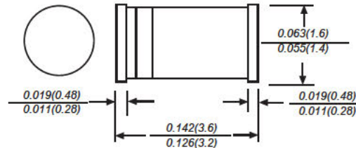
Case: Mini-MELF Dimensions in inches and (millimeters)
