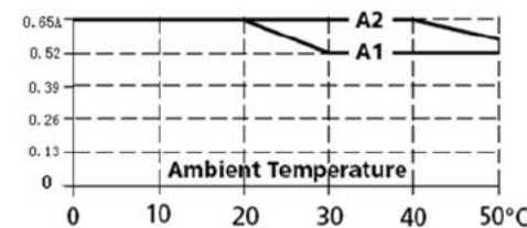
Output Current
