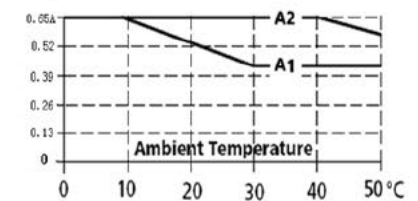
Output Current
