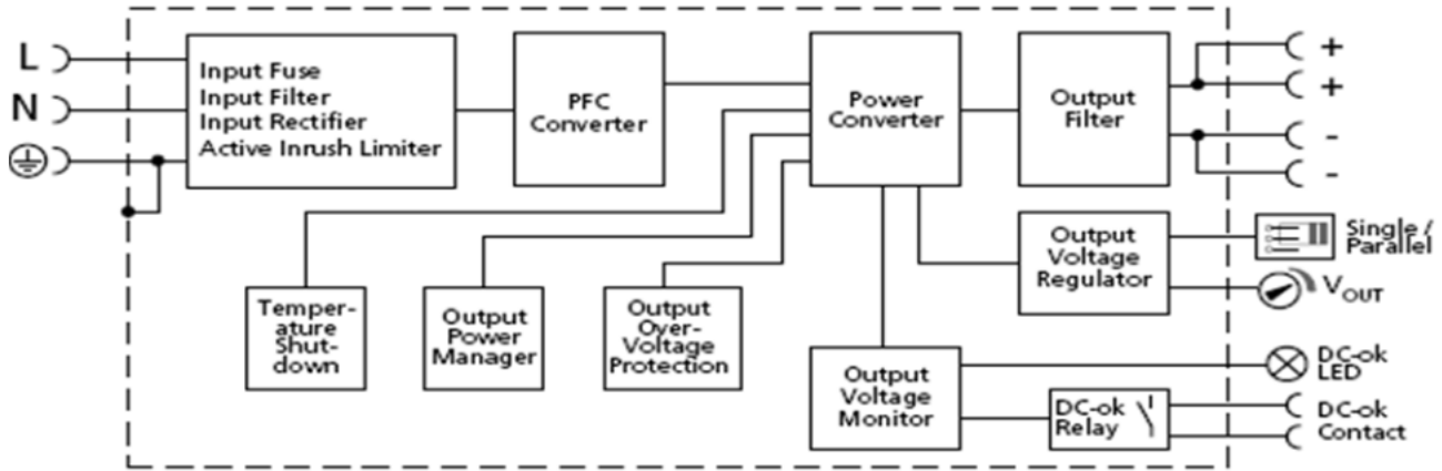
Functional diagram
